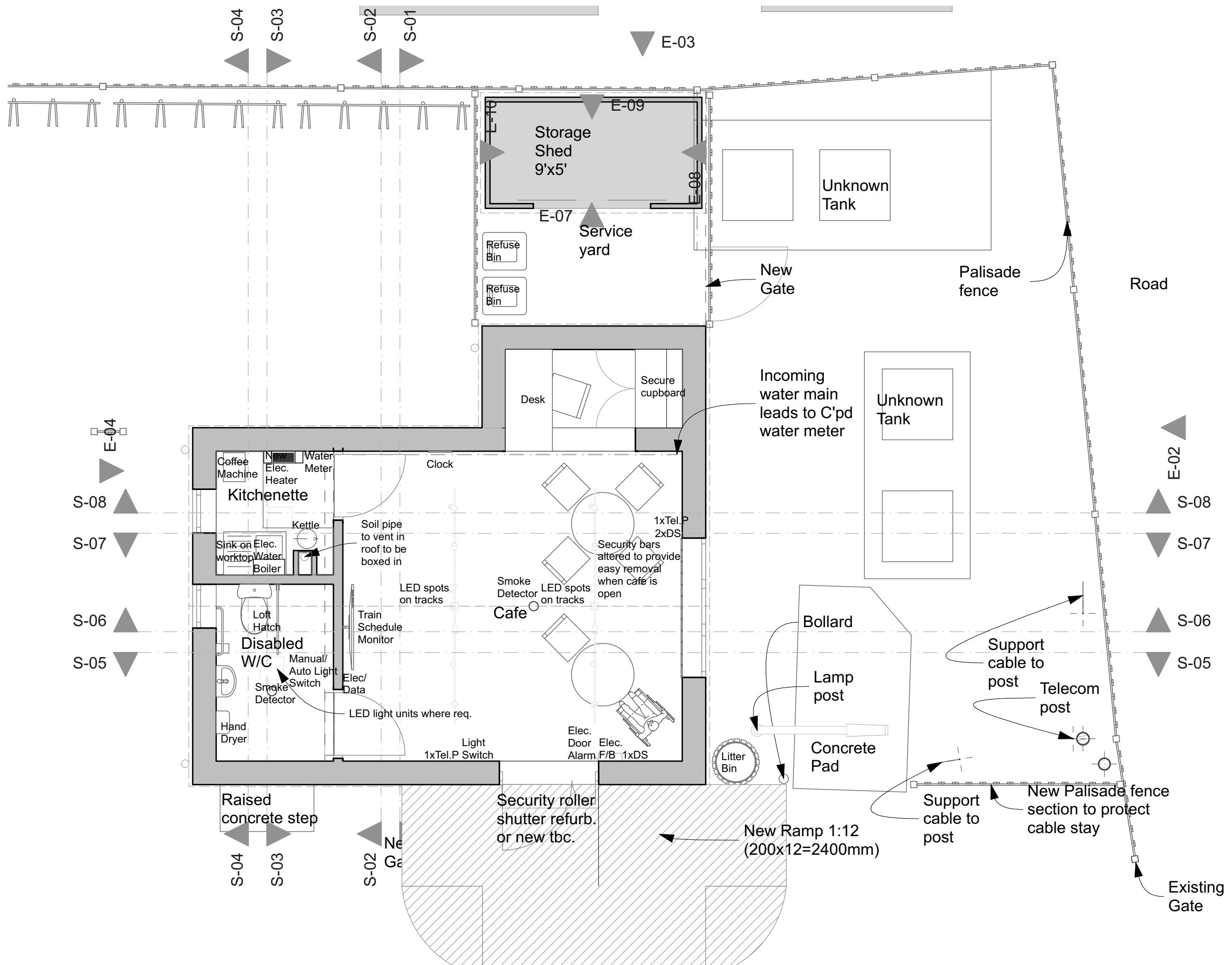
1 GF-Ground Floor Proposed 1:50
